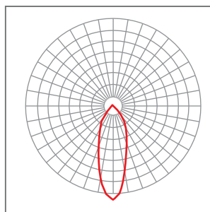
Beam angle 38°
