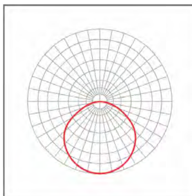
Beam angle 120°
